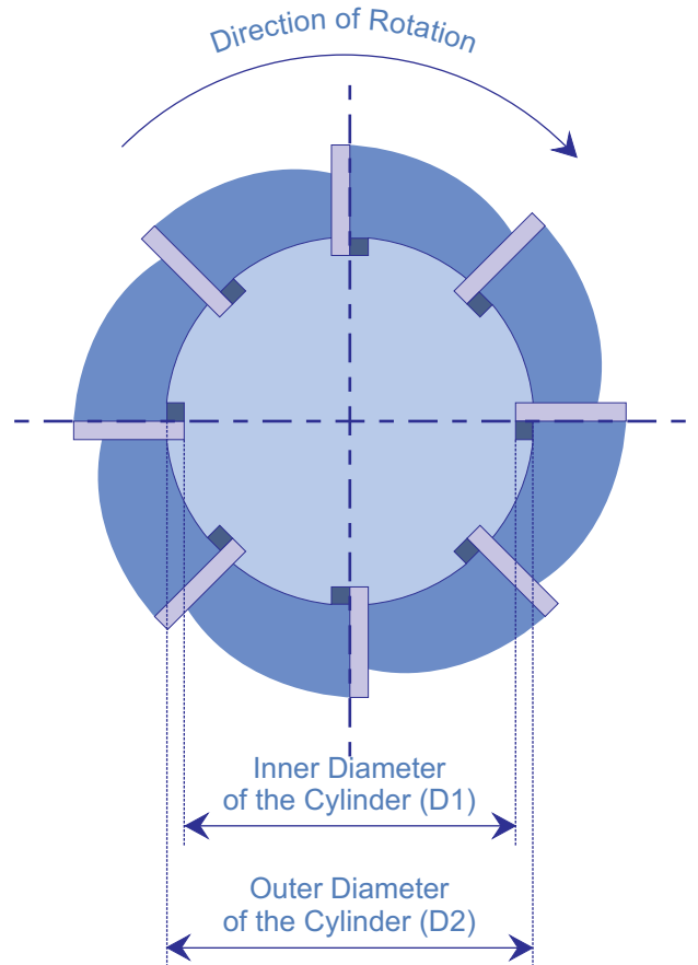
Cross section of the cylinder with 8 blades fitted in its groove
