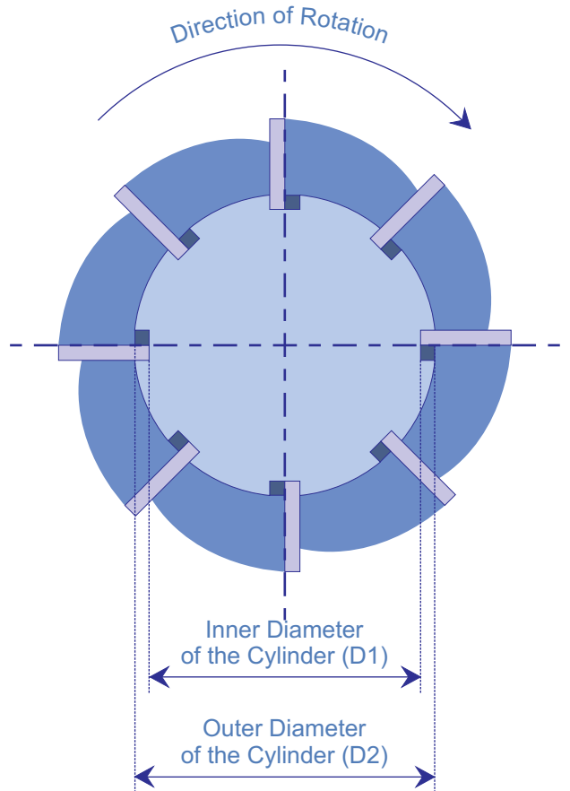
Cross section of the cylinder with 8 blades fitted in its groove
