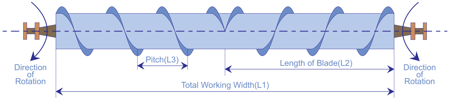
Cylinder with one left hand side blade and one right hand side blade fitted in its groove
